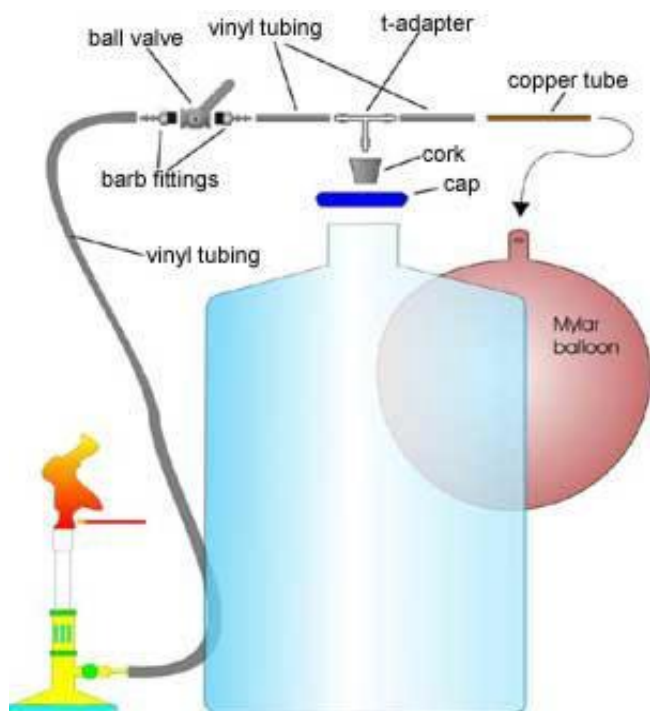
Assembly of the biogas collection system
